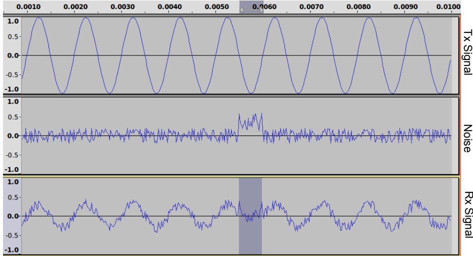
Tx Signal: 1000 Hz sine wave; Attenuation; Random noise with 0.5ms spike
