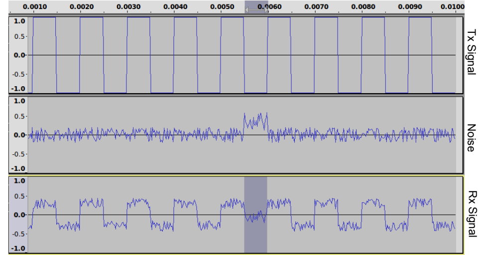
Tx Signal: 1000 Hz square wave; Attenuation; Random noise with 0.5ms spike
